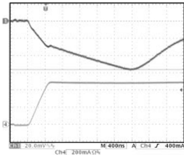
Figure 4–3. No Load – Full Load (500 mA) Transition With C_O = 33\ \mu\text{F} POSCAP™ – Maximum Transient Droop Voltage
