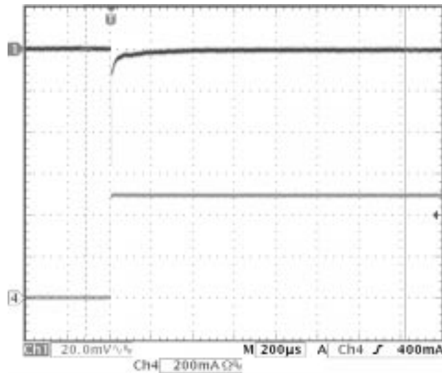
Figure 4–1. No Load – Full Load (500 mA) Transition With C_O = 33\ \mu\text{F POSCAP}^{\text{TM}} – LDO Settling Time
