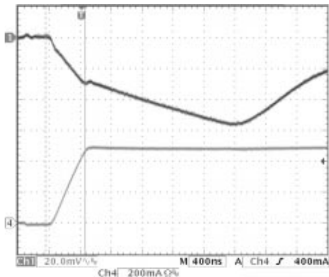
Figure 4–2. No Load – Full Load (500 mA) Transition With C_O = 33\ \mu\text{F POSCAP}^{\text{TM}} – LDO Response Time
